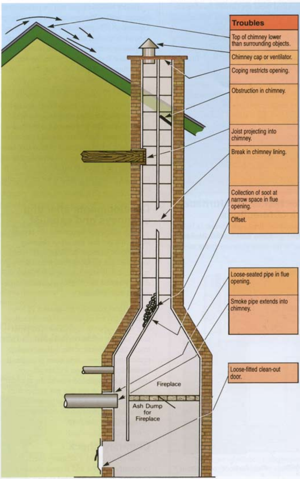
Figure 6-7: Combustion chimney troubles
